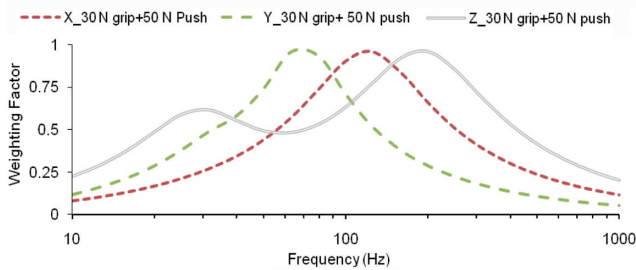
Fig. 5. Finger average VPAD frequency weightings in the three orthogonal directions (X, Y, and Z) derived from the mechanical impedance data reported by Dong et al. 51 .
