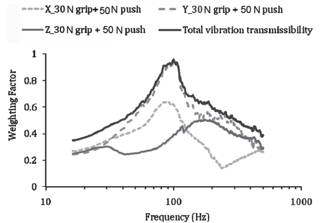
Fig. 10. An example of the profile transmissibility weighting ( W_{Tr-Total-Profile} ) for w_X = w_Y = w_Z = 1 , together with the profile transmissibility weightings in the three directions ( W_{Tr-X-Profile} , W_{Tr-Y-Profile} , and W_{Tr-Z-Profile} ). They are derived from the finger transmissibility measured at several different locations on the fingers 46 .
