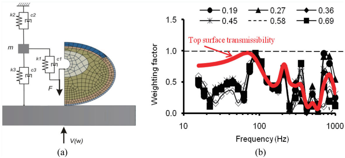
Fig. 6. (a) A finite element model of a fingertip 60 ; and (b) the frequency dependency of the vibration power absorption density at six locations (0.19, 0.27, 0.36, 0.45, 0.58, 0.69 mm) measured from the line 30° from the bone center in the model 60 .
