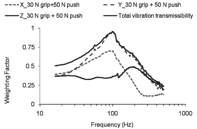
Fig. 9. An example of the total vibration transmissibility weighting ( W_{Tr-Total} ) for w_X = w_Y = w_Z = 1 , together with the relative transmissibility weightings in the three directions ( W_{Tr-X} , W_{Tr-Y} , and W_{Tr-Z} ). They are derived from the finger average transmissibility data reported by Welcome et al. 46 .
