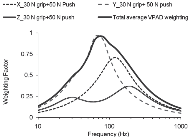
Fig. 8. An example of the total VPAD weighting ( W_{VPAD-Total} ) for w_X = w_Y = w_Z = 1 , together with the relative VPAD weightings in the three directions ( W_{VPAD-X} , W_{VPAD-Y} , and W_{VPAD-Z} ). They are derived from the finger mechanical impedance data reported by Dong et al. 51 .
