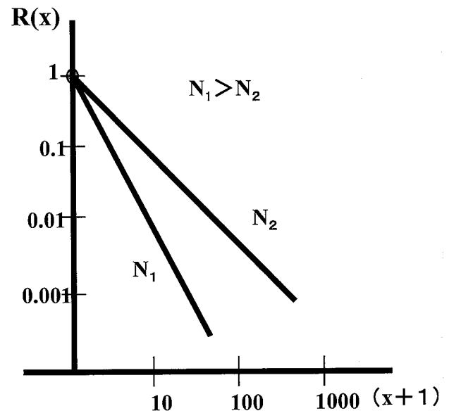
Fig. 5 Schematic figure of normalized risk curve. 正規化リスク曲線の概念図
