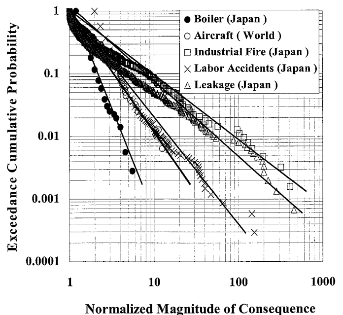
Fig. 7 Normalized risk curves for various types of accidents. 各種災害の正規化リスク曲線
