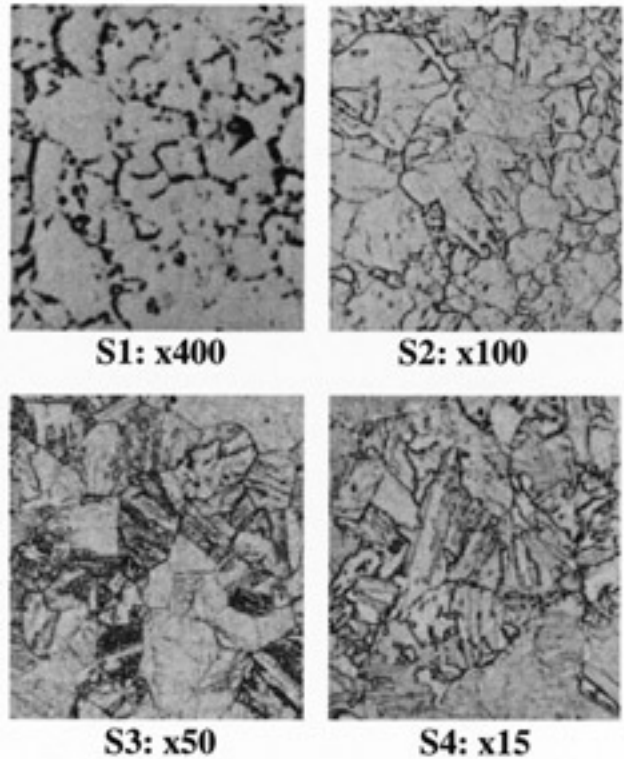
Photo 3 Grain structures of specimens.
