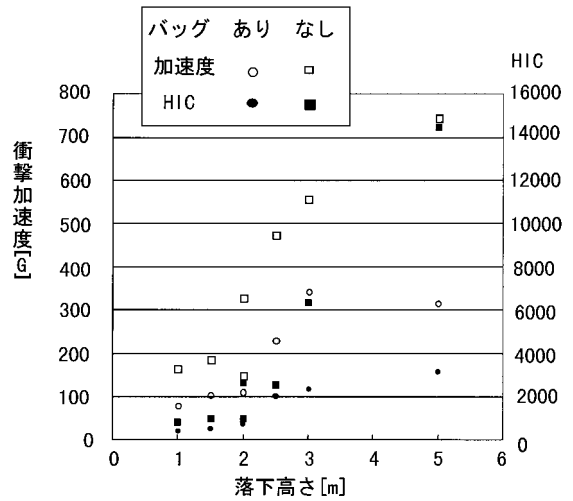
Fig. 8 Shock and fall height. 落下高さや衝撃の大きさ
