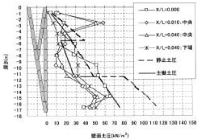
Fig. 28 Distribution of lateral earth pressures on wall (Case15: Crank and rotation about bottom). 壁面土圧の分布状況 (Case15)
