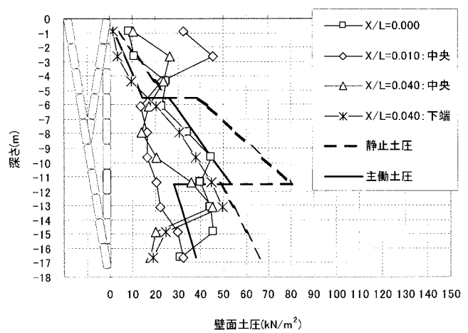
Fig. 31 Distribution of lateral earth pressures on wall (Case18: Crank and rotation about bottom). 壁面土圧の分布状況 (Case18)
