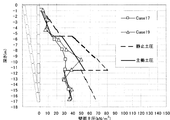
Fig. 35 Distribution of lateral earth pressures on wall. 壁面土圧の分布状況 ( X/L=0.010 : 下端)
