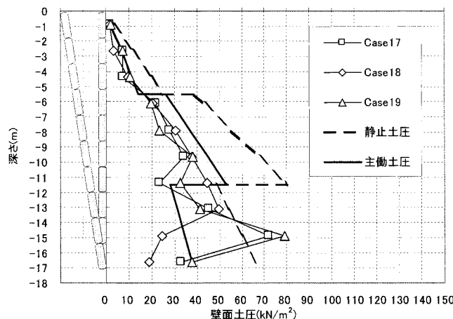
Fig. 36 Distribution of lateral earth pressures on wall. 壁面土圧の分布状況 ( X/L=0.040 : 下端)
