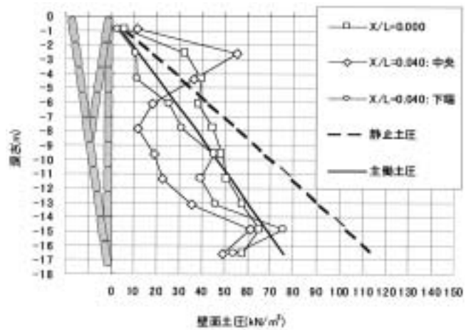
Fig. 17 Distribution of lateral earth pressures on wall (Case6). 壁面土圧の分布状況 (Case6)
