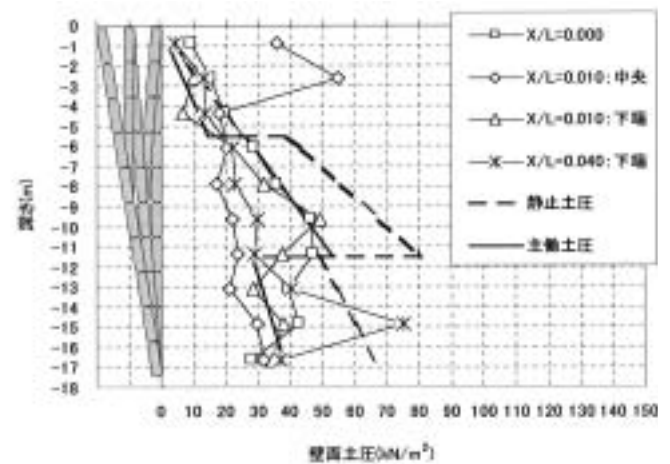
Fig. 32 Distribution of lateral earth pressures on wall (Case19: Rotation about bottom and crank by repetition). 壁面土圧の分布状況 (Case19)
