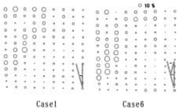
Fig. 9 Distributions of maximum shear strain ( \gamma_{max} ) ( X/L=0.1 ) . 最大せん断ひずみ分布 ( X/L=0.1 )
