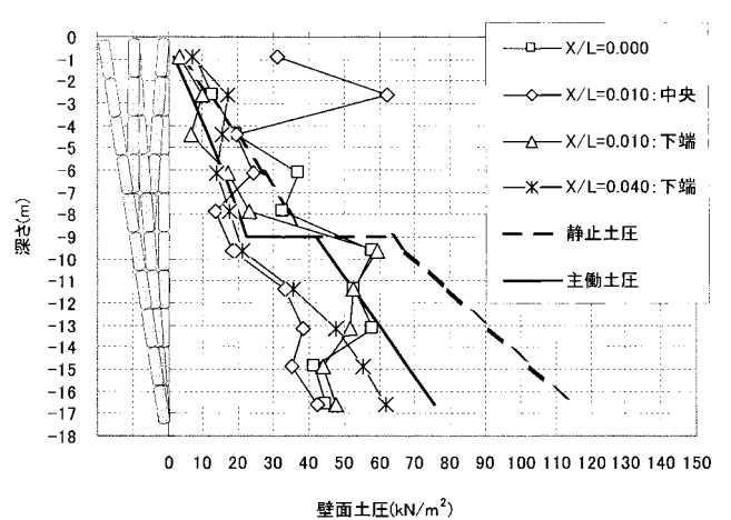
Fig. 26 Distribution of lateral earth pressures on wall (Case13: Rotation about bottom and crank by repetition). 壁面土圧の分布状況 (Case13)
