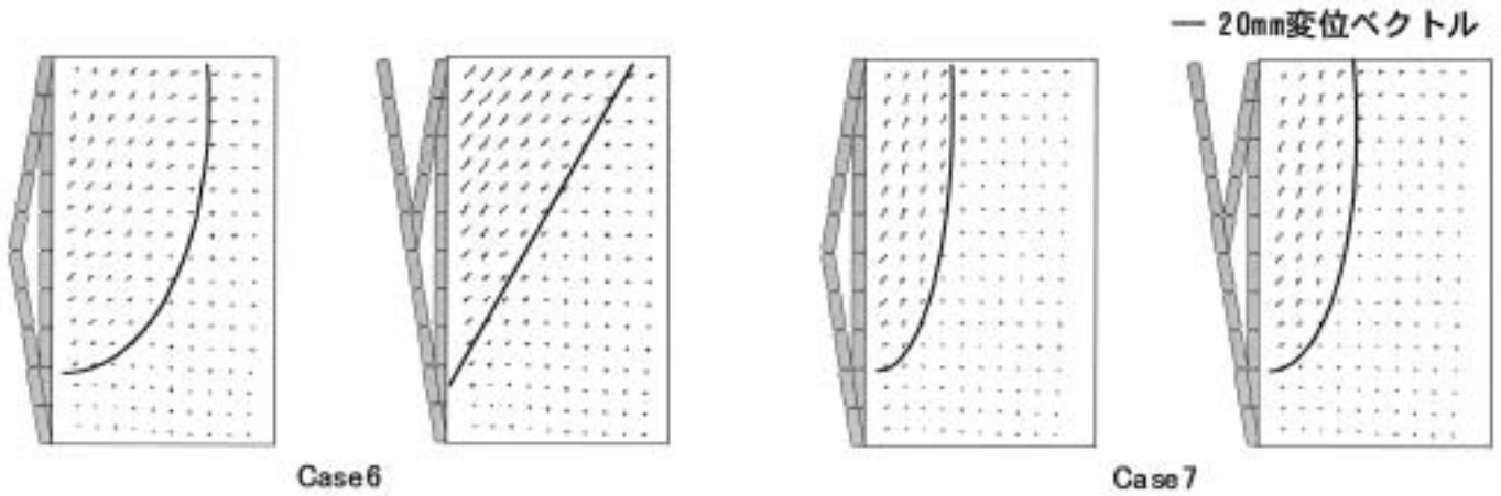
Fig. 16 Displacements of model grounds in Case6 and Case10 ( X/L=0.04 ). 背面地盤の変位状況 ( X/L=0.040 )
