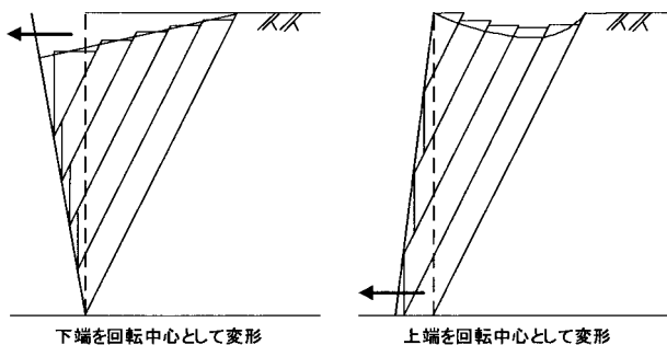
Fig. 12 Ground movements caused by the wall deflection. 土留め壁の変形に伴う砂層の変位
