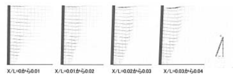
Fig. 6 Visualized deformation area in Case2 (rotation about top). 変位領域の可視化画像 (Case2)
