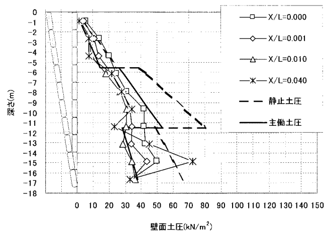
Fig. 30 Distribution of lateral earth pressures on wall (Case17: Rotation about bottom). 壁面土圧の分布状況 (Case17)
