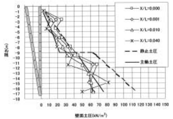
Fig. 24 Distribution of lateral earth pressures on wall (Case11:Rotation about bottom). 壁面土圧の分布状況 (Case11)
