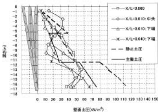
Fig. 29 Distribution of lateral earth pressures on wall (Case10: Rotation about bottom and crank by repetition). 壁面土圧の分布状況 (Case16)
