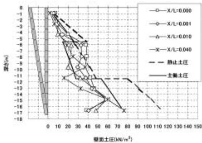
Fig. 27 Distribution of lateral earth pressures on wall (Case14: Rotation about bottom). 壁面土圧の分布状況 (Case14)
