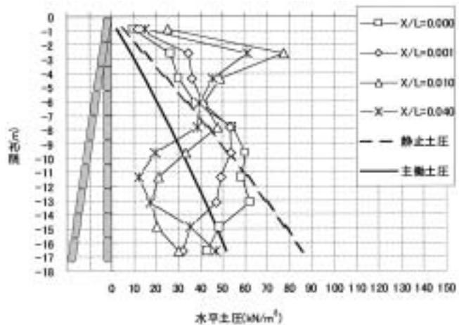
Fig. 11 Distribution of lateral earth pressures on wall (Case2 : Rotation about top). 壁面土圧の分布状況 (Case2)
