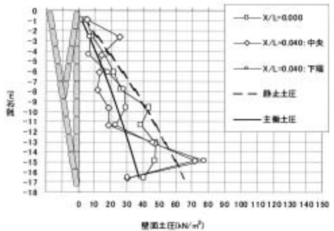
Fig. 18 Distribution of lateral earth pressures on wall (Case7). 壁面土圧の分布状況 (Case7)
