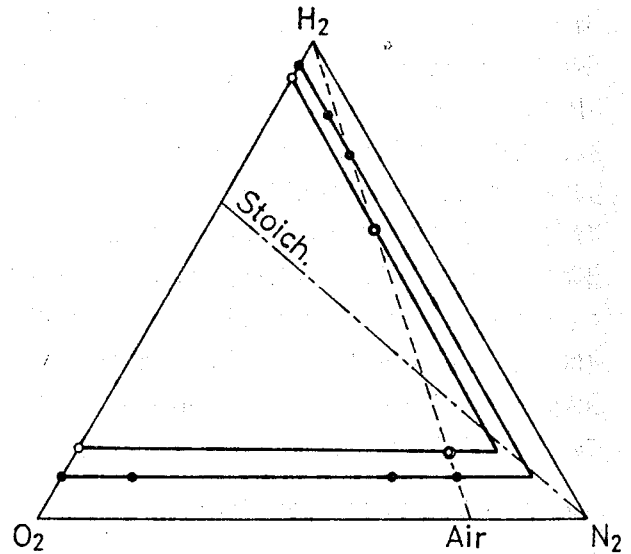
Fig. 10 Detonability limits in H 2 -O 2 -N 2 mixtures ● results for infinite tube obtained by extrapolation by Wagner, Ref. 3 ○ results in 1 inch tube, detonation initiated by 2H 2 +O 2 detonation, by Munday, Ref. 1 ◎ Present results in 1 inch tube, detonation initiated by 2H 2 +O 2 detonation
