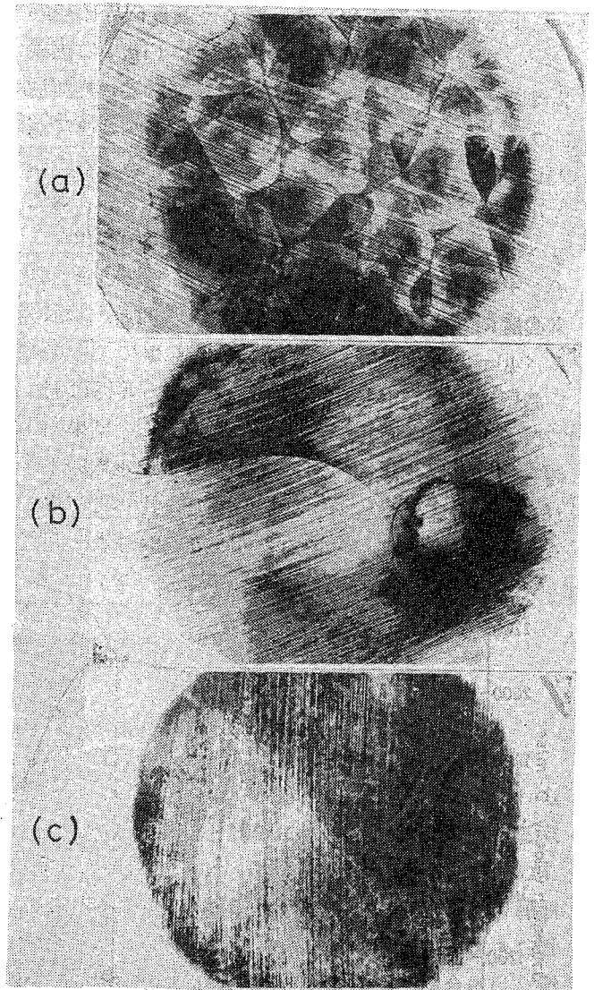
Fig 4 Soot track records of transverse wave structure in hydrogen-air detonations taken on the end plate of 1inch tube. (a) : multi-head structure, (b) : single-spin structure, (c) : overdriven structure by reflected shock wave
