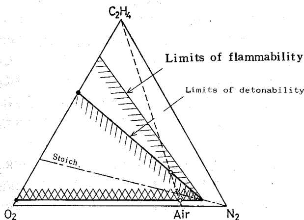
Fig. 11 Limits of flammability and detonability in C 2 H 4 -O 2 -N 2 mixtures
