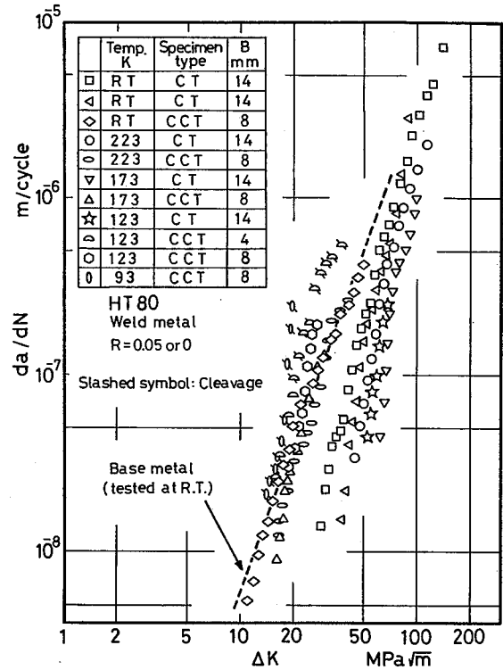
Fig. 4 Relation between fatigue crack growth rates and \Delta K in welds at temperatures ranging from room temperature down to 93 K. 室温から 93 K の範囲の溶接部の疲労き裂伝播速度と \Delta K の関係
