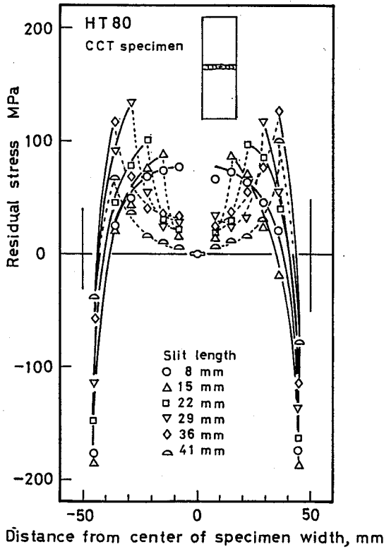
Fig. 7 Redistributions of residual stresses in welds in CCT specimen. CCT 試験片の溶接部の残留応力の再分布
