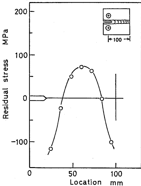
Fig. 8 Residual stress distribution in welds in CT specimen. CT 試験片の溶接部の残留応力分布
