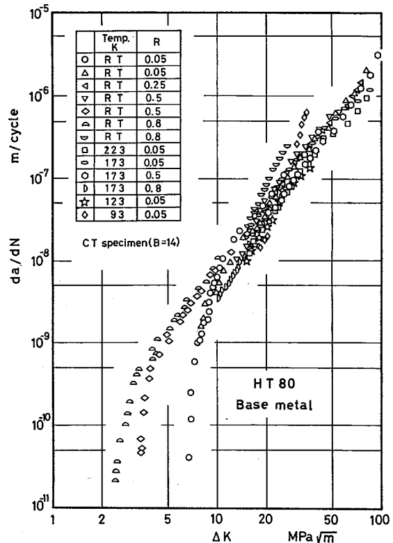
Fig. 2 Relation between fatigue crack growth rates and \Delta K in base metal at temperatures ranging from room temperature down to 93 K.
