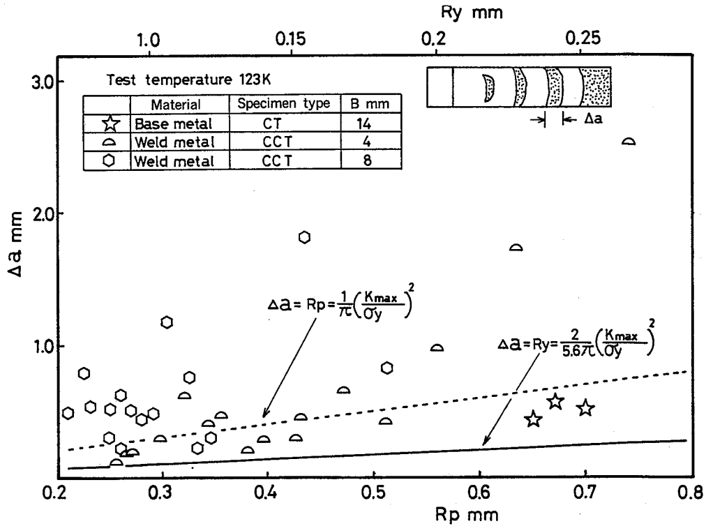
Fig. 6 Relation between width of cleavage, \Delta a , and plastic zone size, R_y . へき開の幅 \Delta a と塑性域寸法 R_y の関係。
