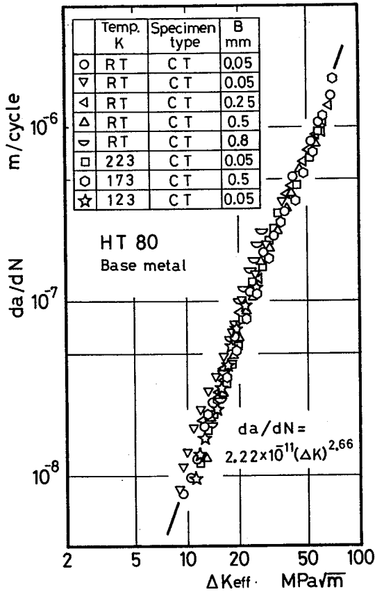
Fig. 9 Relation between fatigue crack growth rates and \Delta K_{eff} in base metal at temperatures ranging from room temperature down to 123 K. 室温から 123 K の範囲の母材の疲労き裂伝播速度と \Delta K_{eff} の関係
