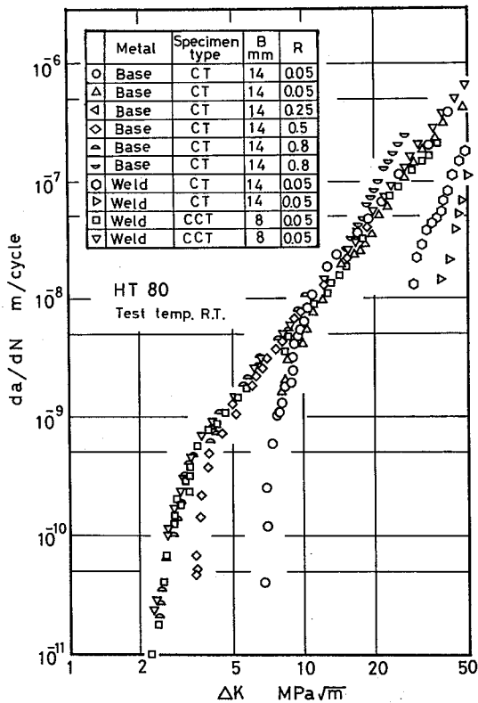
Fig. 3 Comparison of fatigue crack growth rates between base metal and welds at room temperature. 室温における母材と溶接部の疲労き裂伝播速度の比較。
