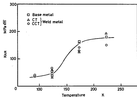
Fig. 11 Relation between fatigue fracture toughness which is taken into account residual stresses, K_{fcR} , and temperature.
