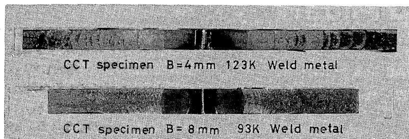
Photo.1 Fractographs showing cyclic cleavage occurred during fatigue crack growth under low temperatures.
