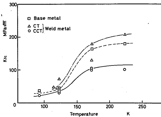
Fig. 5 Effect of temperature on fatigue fracture toughness in base metal and welds.
