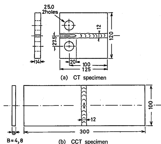
Fig. 1 Configurations of specimens used. 試験片の形状
