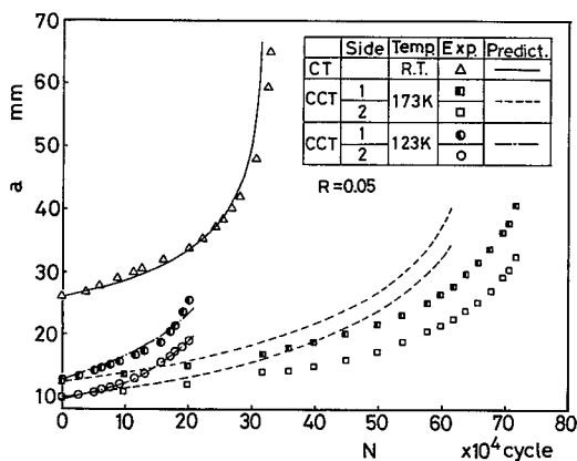
Fig. 12 Prediction of fatigue crack growth lives in welds with residual stresses. 残留応力を有する溶接部の疲労き裂伝播寿命の予測
